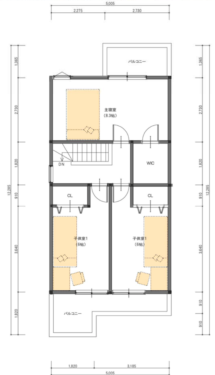
2F PLAN
